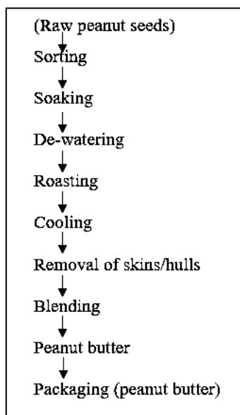
Figure 1: Preparation of peanut butter Source: Olawuni et al. , (2019)
