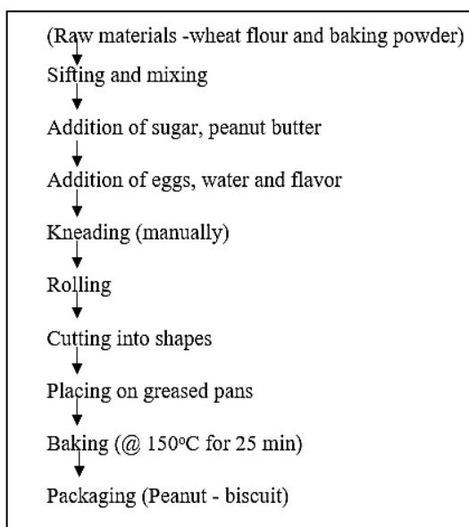
Figure 2: Production of biscuits from wheat flour and peanut butter (Modified method). Source: (Peter-Ikechukwu et al. , 2017)
