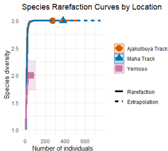
Figure 2: Species Refraction Curves by locations
