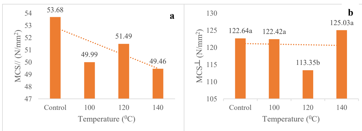
Figure 1: Effect of temperature on the (a) Maximum Compressive Strength parallel to grain of Pinus caribaea wood, and (b) Maximum Compressive Strength Perpendicular to grain of Pinus caribaea wood
