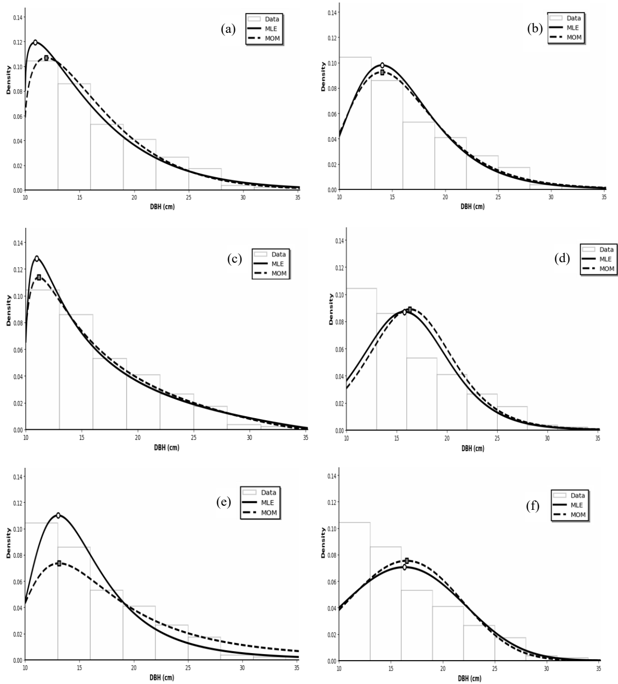
Figure 2(a-f): Probability Density Function Comparison between Methods of Moments and Maximum Likelihood Estimation Approach for 3-P Weibull (a); Gumbel (b); Johnson's SB (c); Logistic (d); Generalized Extreme Value (e) and 2-P Weibull (f)
