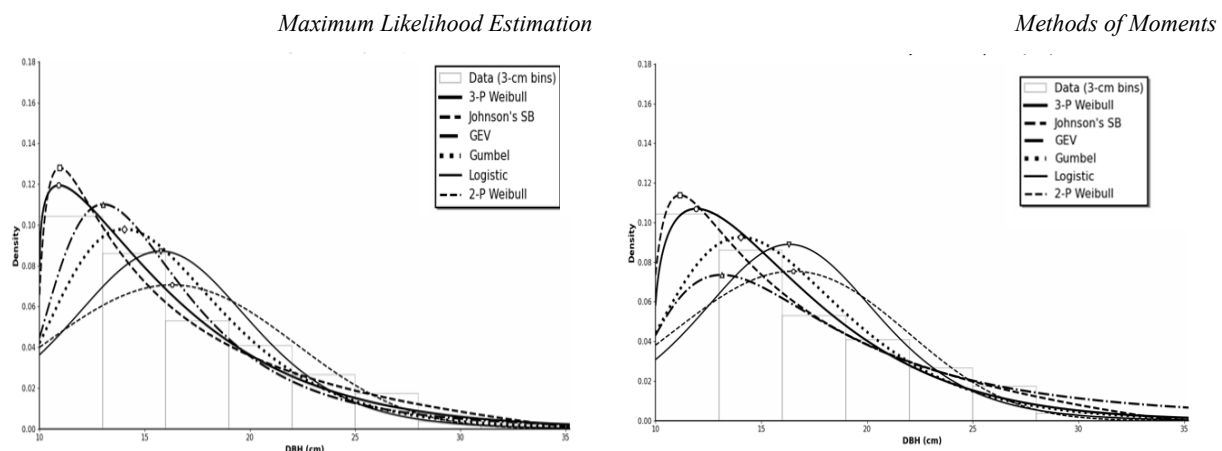
Figure 1: Diameter Distribution Probability Density Function Comparison
