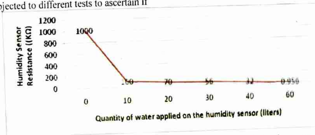
Fig. 12 Graph of humidity sensor resistance against the quantity of water applied on the gypsum.
