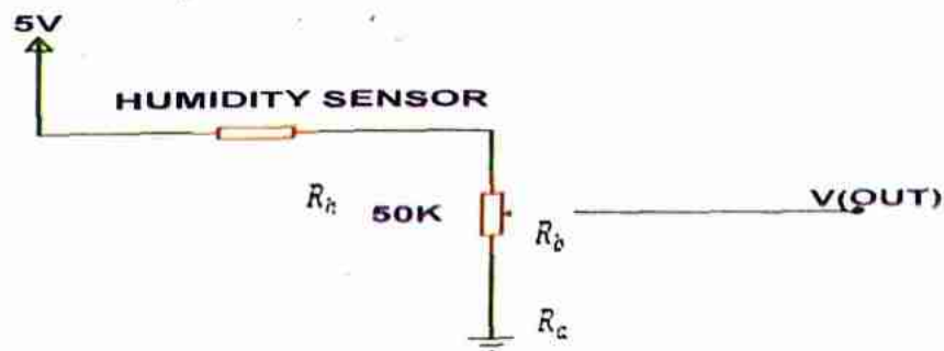
Fig. 2 Circuit diagram of humidity sensor.
