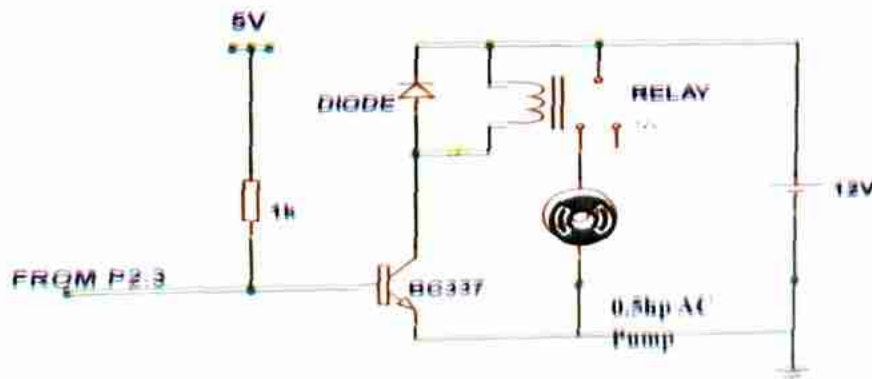
Fig. 8 Schematic representation of electric motor circuit.
