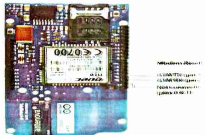
Fig. 10 Pin Outs of The Arduino GSM Shield
