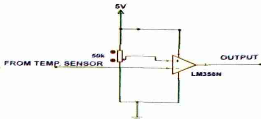
Fig. 5 Schematic capture of temperature sensor comparator circuit.
