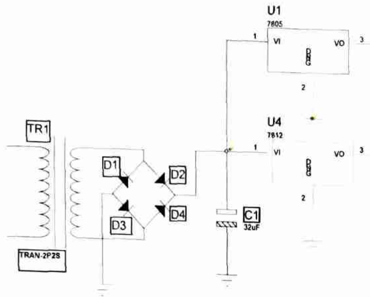
Fig. 1 DC Power Supply.
