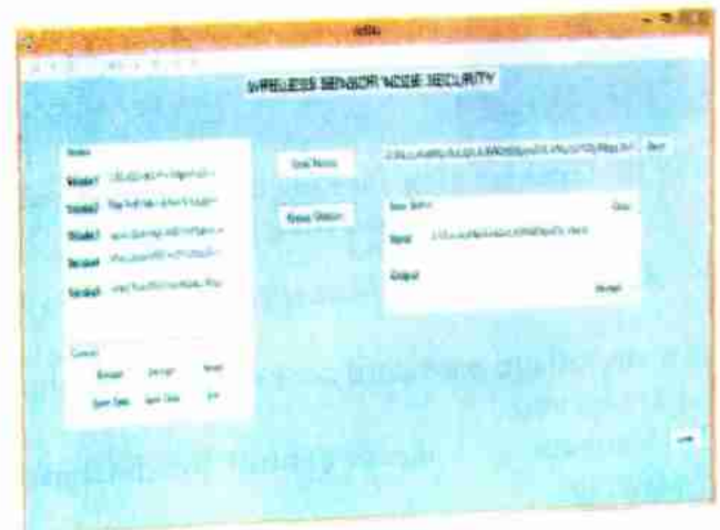
Fig 7: Encryption Simulation.
