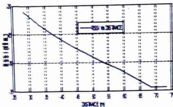
Fig. 4: Average values of RSSI versus Distance
