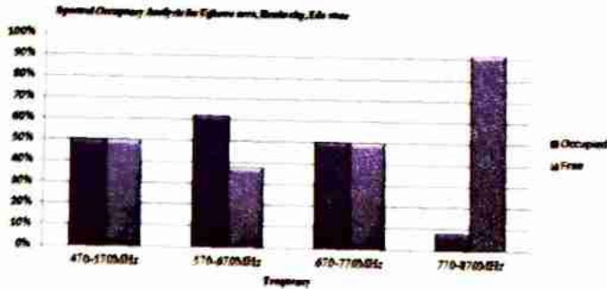
Figure 6: Spectrum occupancy in Ugbowo area, Benin City, Edo State.
