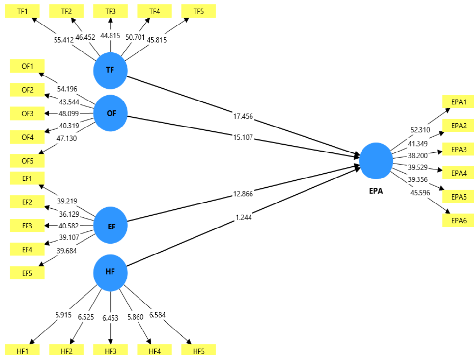
Figure 4: Bootstrapped t-values
