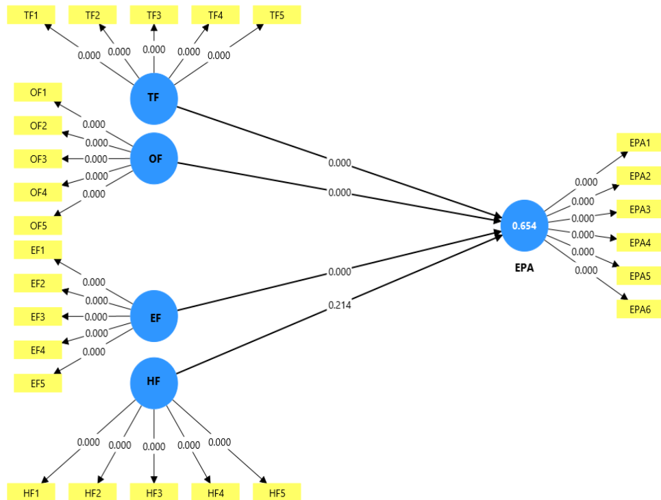
Figure 3: Bootstrapped p-values
