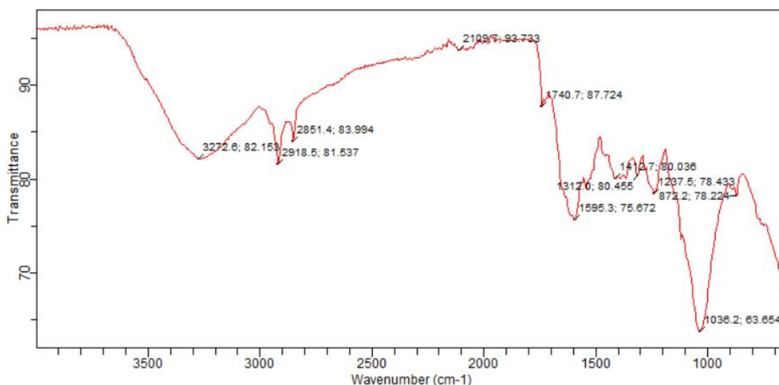
Fig 1: Showing the FTIR of the extracted Irvingia gabonensis mucilage
