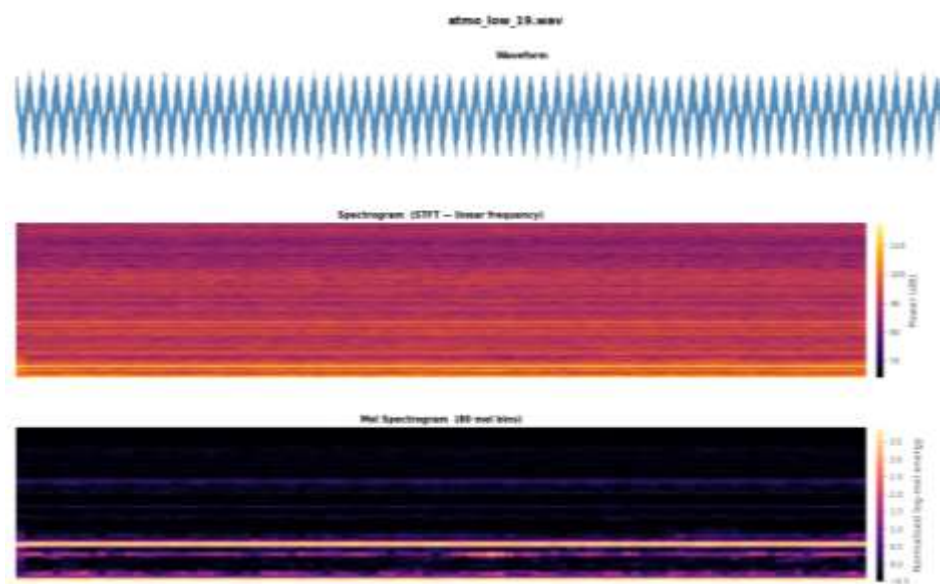
Figure 23: Visualization of Inference Audio Data Processing
