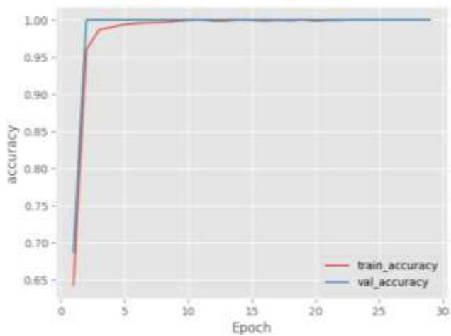
Figure 20: cnn2d_model Accuracy
