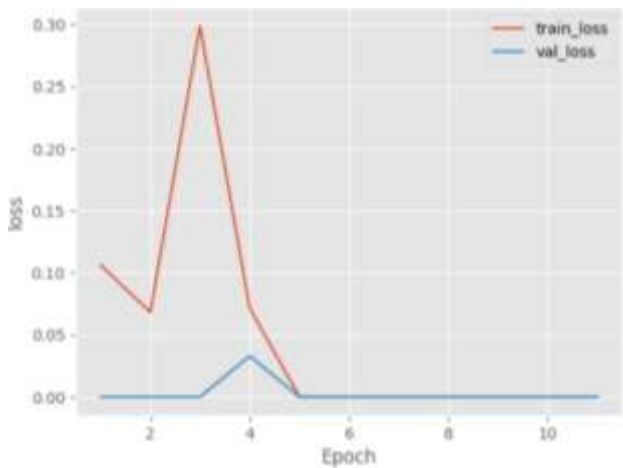
Figure 16: Sinusoidal_pe Loss
