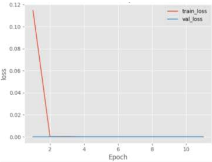
Figure 13: Rotational_pe Loss
