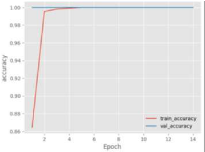
Figure 2: GRU Accuracy
