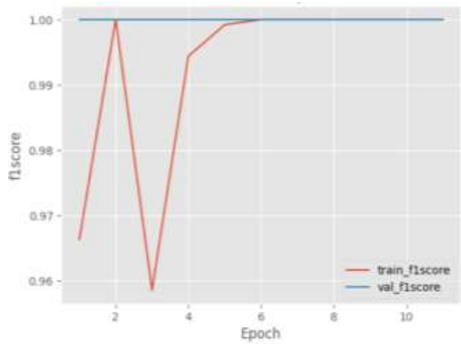
Figure 18: Relative_pe F1-Score
