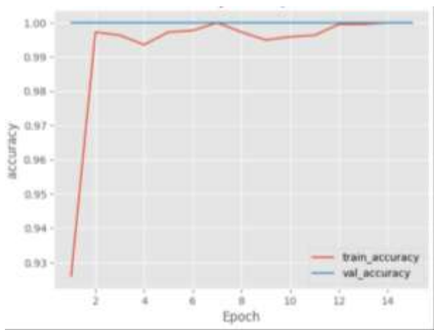
Figure 5: LSTM Accuracy
