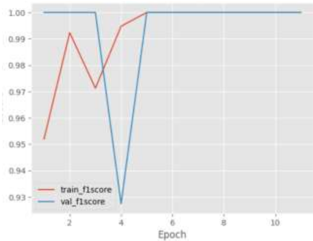
Figure 15: Sinusoidal_pe F1-Score
