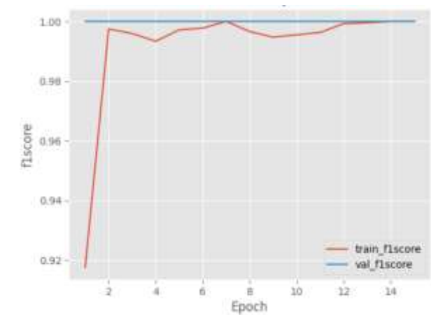
Figure 6: LSTM F1-Score
