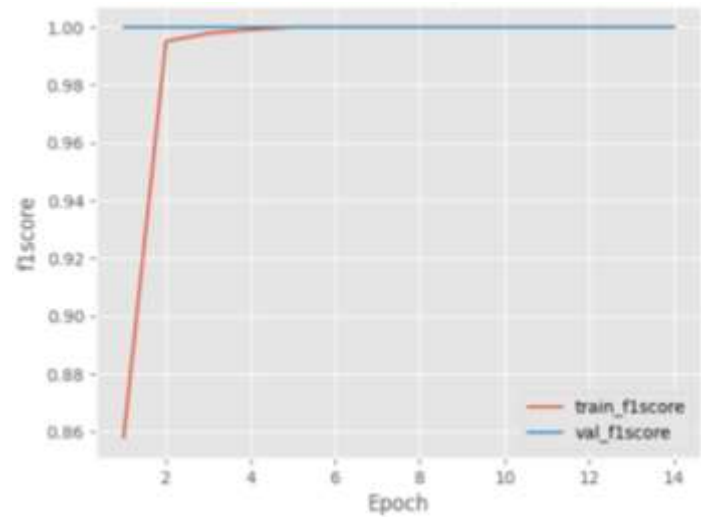
Figure 3: GRU F1-Score
