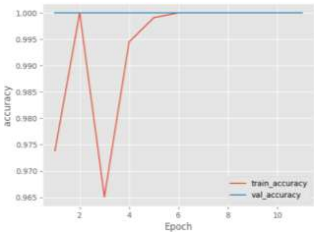
Figure 17: Relative_pe Accuracy
