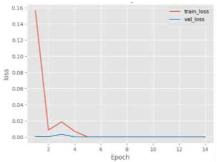
Figure 10: LSTM-GRU Loss
