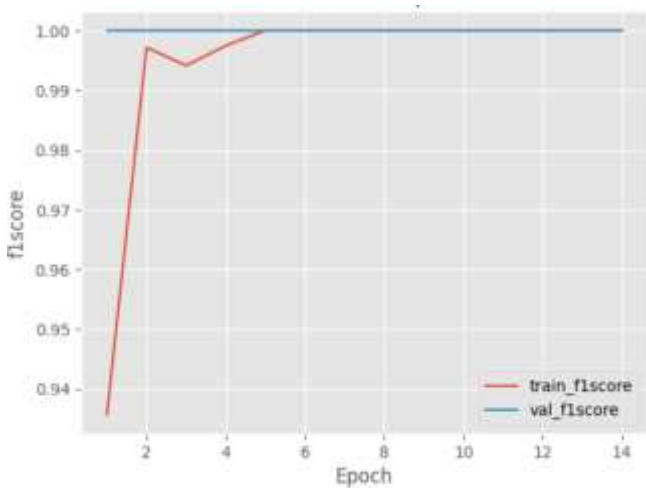
Figure 9: LSTM-GRU F1-Score
