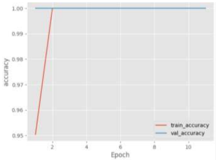
Figure 11: Rotational_pe Accuracy
