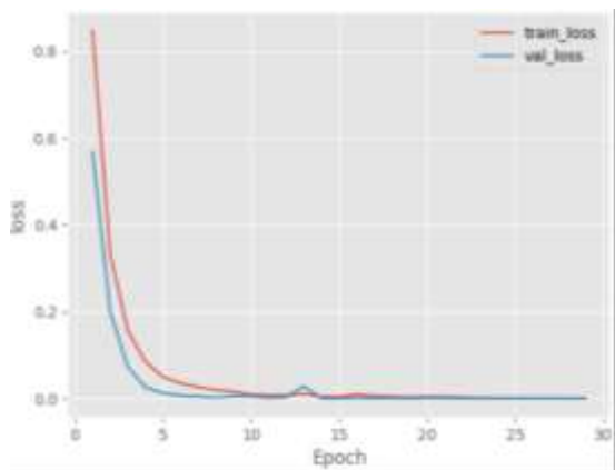
Figure 22: cnn2d_model Loss
