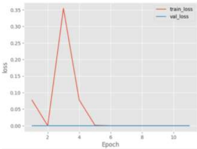
Figure 19: Relative_pe Loss
