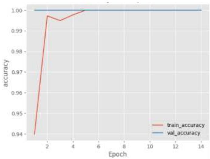
Figure 8: LSTM-GRU Accuracy
