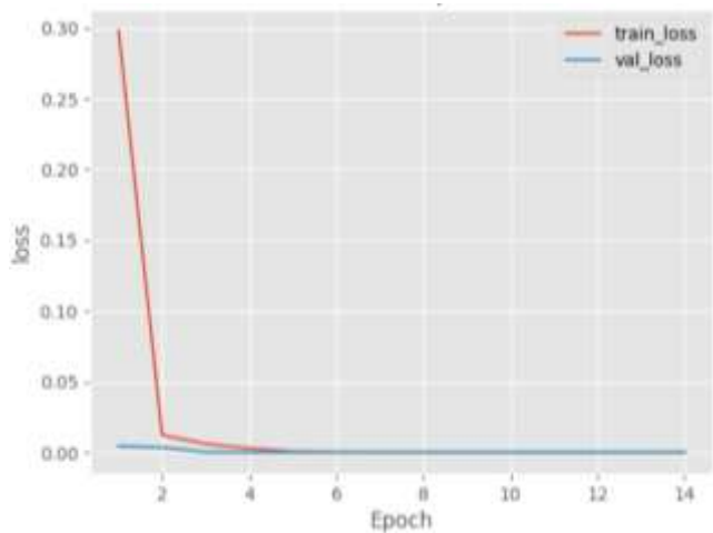
Figure 4: GRU Loss
