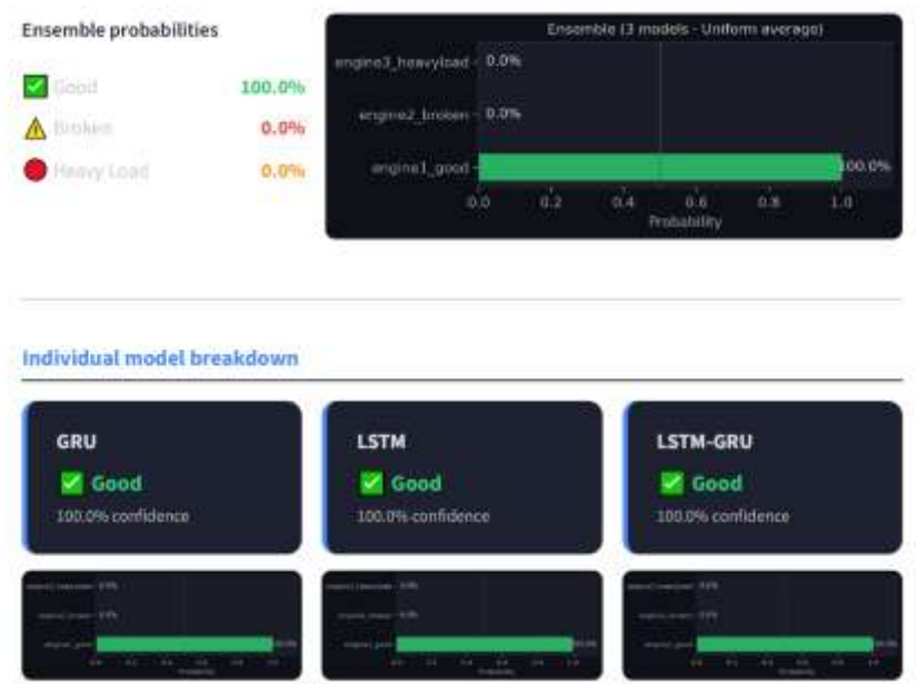
Figure 25: Recurrent Model Performances
