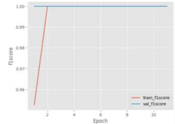
Figure 12: Rotational_pe F1-Score
