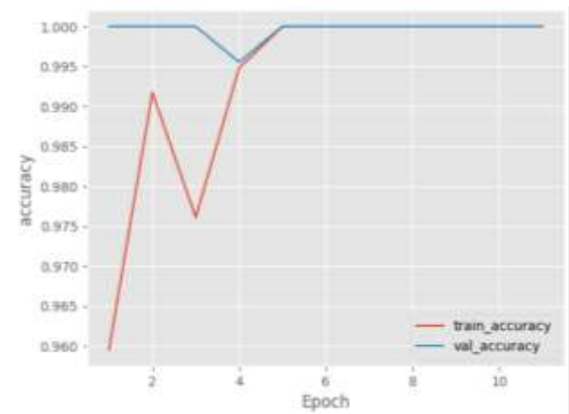
Figure 14: Sinusoidal_pe Accuracy
