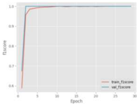
Figure 21: cnn2d_model F1-Score
