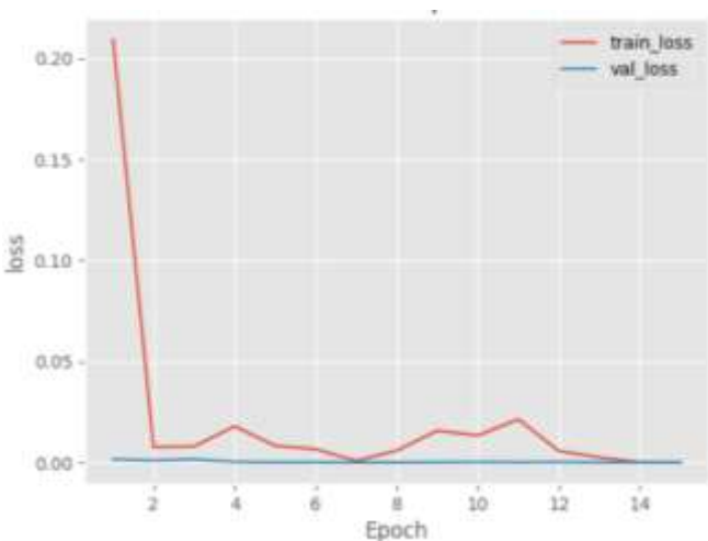
Figure 7: LSTM Loss
