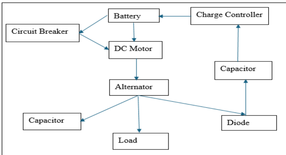
Figure 1. A simplified flow chart of the design of the CFF generator
