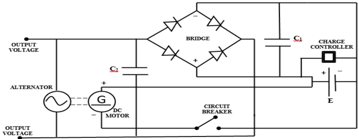
Figure 2. Schematic diagram of the CFF generator with symbols of the components Having used the schematic diagram to construct the CFF generator, the actual physical structure of the generator is shown in figure 3.
