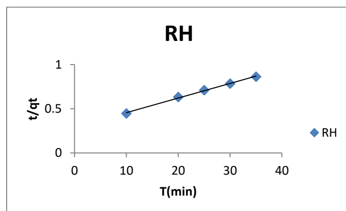
Figure 8: Linear pseudo second order kinetic plot
