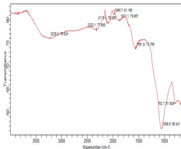
Figure 1: FTIR spectra of RH before adsorption
