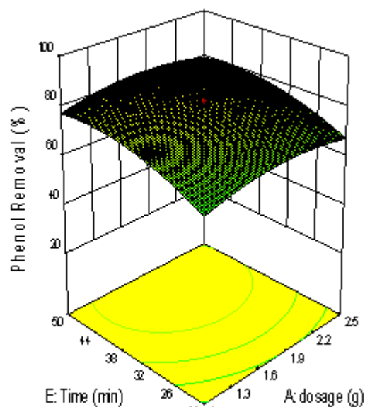
Figure 20. 3D plot of the effect of contact time and adsorbent Dosage
