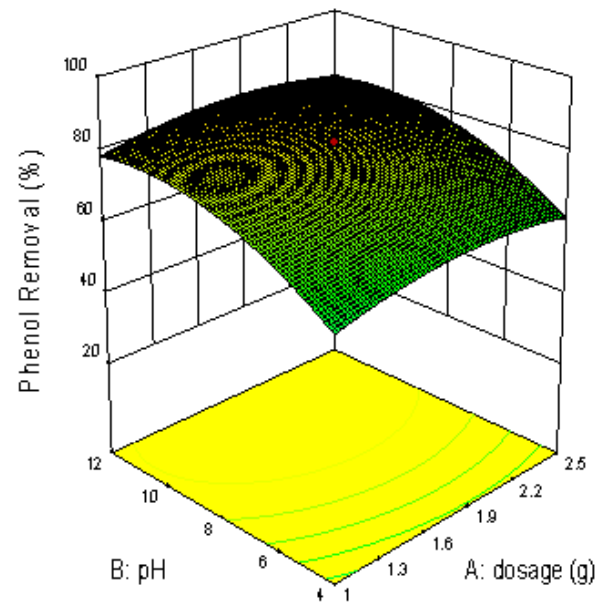
Figure 15. 3D plot of the effect of pH and adsorbent dosage
