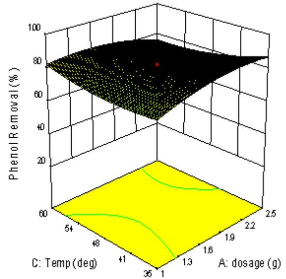
Figure 14. 3D plot of the effect of Effluent temperature and adsorbent dosage
