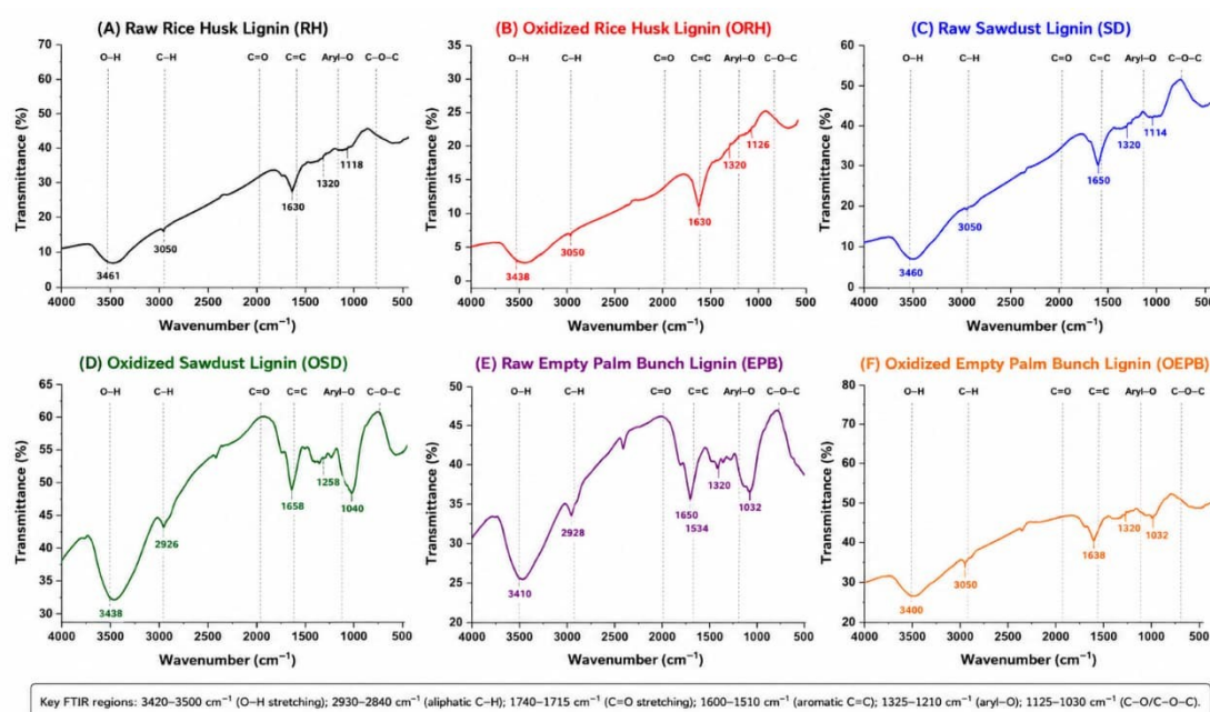
Figure 2. FTIR spectra of raw and oxidized lignin samples derived from rice husk (RH), sawdust (SD), and empty palm bunch (EPB).
