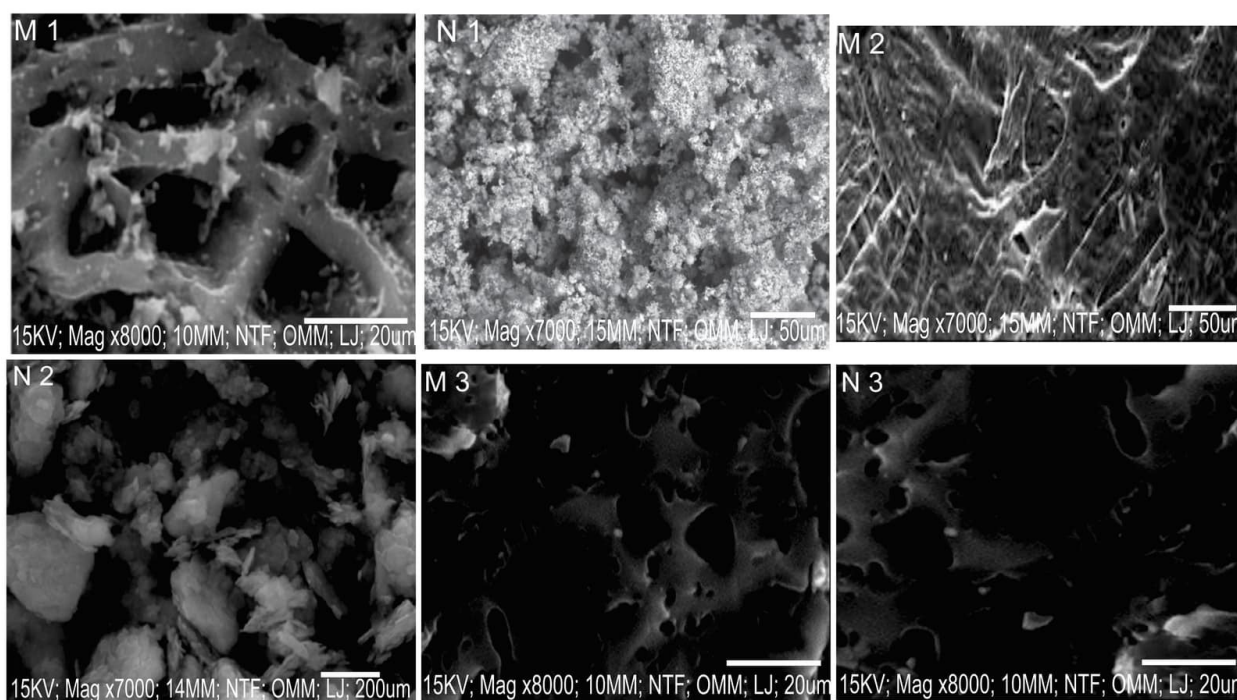
Figure 3: SEM combined panel (raw vs oxidized for RH, SD, EPB).
