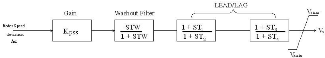
Fig. 6: Transfer functions of the PSS model, where K_{pss} is a constant gain, and all T_s are time constants. The first block is the stabilizer gain block with the constant gain K_{pss} , which determines the amount of damping. The second block is the washout filter, which serves as a high-pass filter, with a time constant that allows the signals associated with oscillations in rotor speed to pass unchanged, and does not allow the steady state changes to modify the terminal voltages. The last block, the phase-compensation, provides the desired phase-lead characteristic to compensate for the phase lag between the AVR input and the generator electrical (air-gap) torque.
