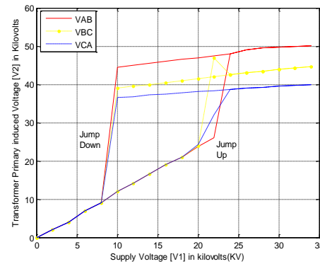
Fig. 4. Graph of primary terminal voltage against supply voltage at no load.
