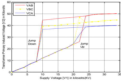
Fig. 6. Graph of primary induced voltage against supply voltage at no-load during unsymmetrical switching of the transformer.
