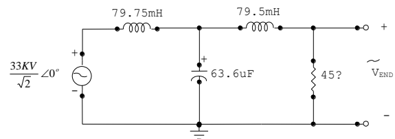
Fig. 2.0. Ferranti rise in cable under load condition.
