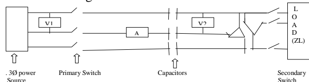
Fig. 3. Ferroresonant experiment circuit for 3 Ø DY11 transformer.
