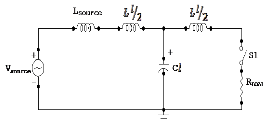
Fig. 1. Equivalent circuit of 1-phase conductor for the calculation of Ferranti rise.
