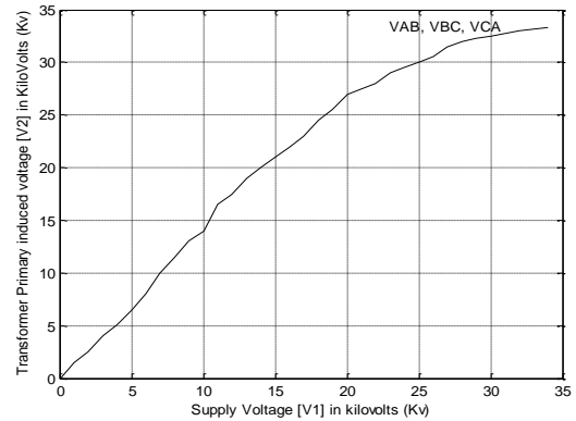
Fig. 8. Graph of primary induced voltages against supply voltages when the transformer is on-load.
