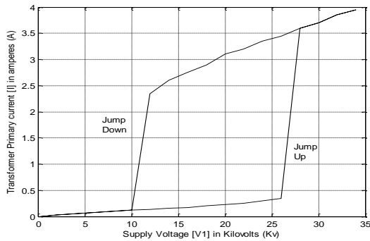
Fig. 7. Graph of Primary induced current versus supply voltage at no-load during unsymmetrical switching of the transformer.
