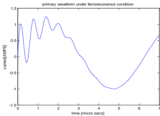
Fig.11. Distortion of primary waveform due to ferroresonance.
