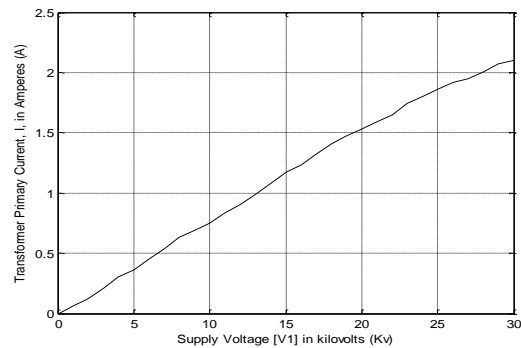
Fig. 9. Graph of Primary induced current versus supply voltages when the transformer is on-load.
