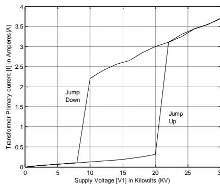
Fig. 5. Graph of Primary induced current versus supply voltage at no-load.
