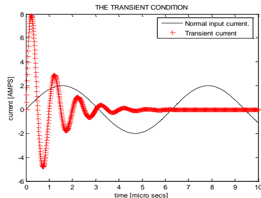
Fig.10. Primary normal current and the switching in-rush current (due to ferroresonance) of the transformer plotted at the same time base.
