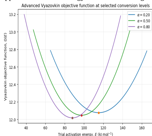
Figure 5. Advanced Vyazovkin objective functions at selected conversion levels.
