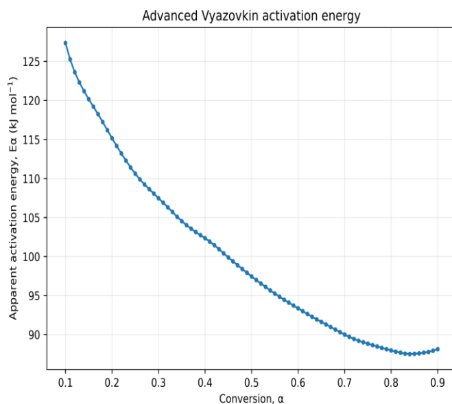
Figure 6. Apparent activation energy as a function of conversion for Cerbera odollam seed oil.
