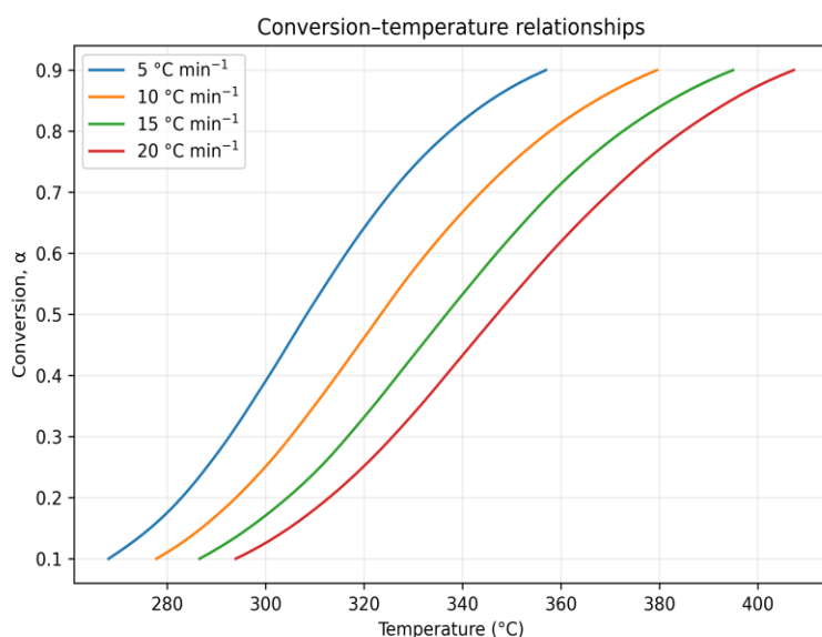
Figure 4. Conversion–temperature profiles of Cerbera odollam seed oil at different heating rates.
