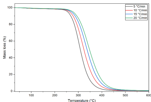
Figure 2. Thermogravimetric (TGA) curves of Cerbera odollam seed oil at different heating rates.
