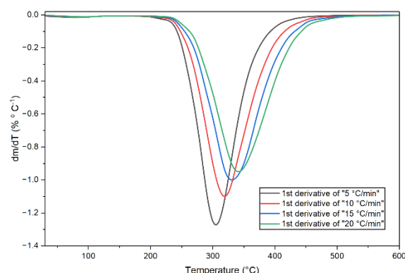
Figure 3. Derivative thermogravimetric (DTG) curves of Cerbera odollam seed oil at different heating
