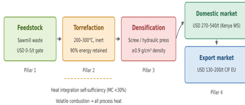
Figure 2: Torrefaction-densification value chain: process stages, four cost pillars, and market endpoints
