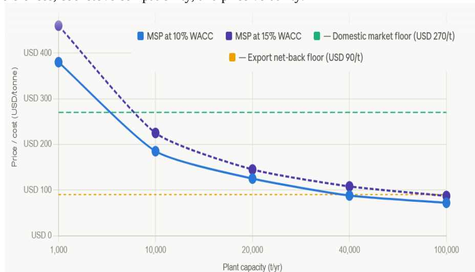
Figure 4: SSA-adjusted minimum selling price versus plant scale, with domestic and export market price reference thresholds
