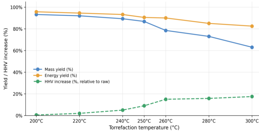
Figure 3: Mass yield, energy yield, and HHV increase of woody biomass as a function of torrefaction temperature (sources: Simonic et al., 2020; Tumuluru et al., 2011; Poudel et al., 2018)
