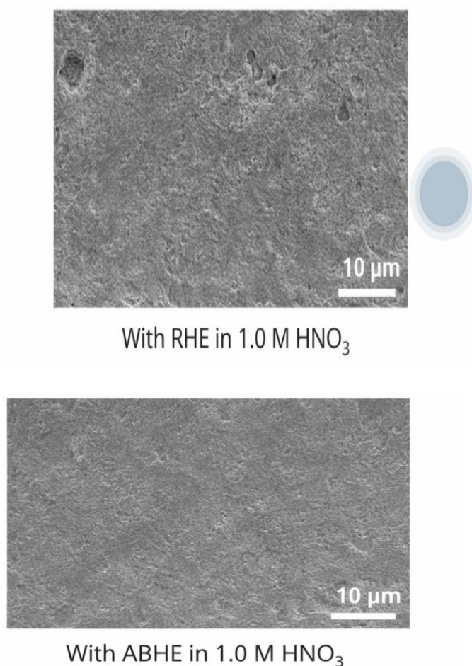
Figure 5: Scan electron microscopy micrograph of the mild steel
