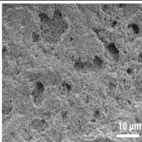
Uninhibited in 1.0 M \text{HNO}_3
