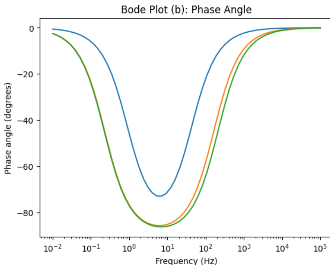
Figure 4(b): Bode phase angle shows a lower and narrower phase-angle peak, indicating active corrosion. RHE and especially ABHE display a broader phase-angle maximum approaching -80^\circ , indicating capacitive behaviour and the formation of a stable, adsorbed protective film. The ABHE's higher and wider peak supports its slightly superior inhibition efficiency.
