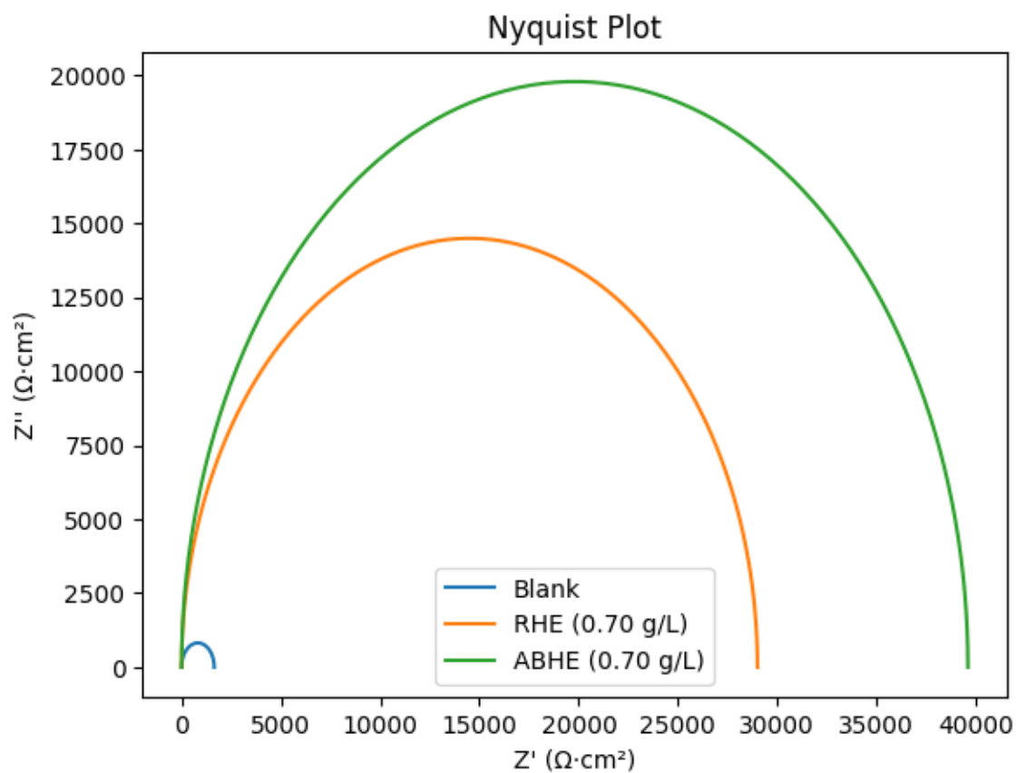
Figure 3: Nyquist plots for mild steel in 1.0 M \text{HNO}_3 without inhibitor and with RHE and ABHE at selected concentrations,
