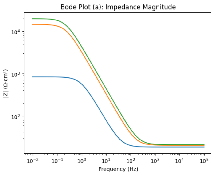
Figure (4a) : Bode impedance magnitude shows much higher |z| values at low frequencies compared to the blank, which indicates barrier protection. The high-frequency convergence reflects solution resistance.
