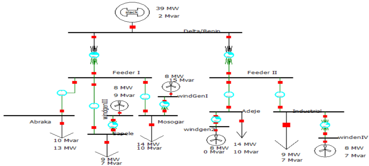
Figure 2: integration of wind turbine to the network.
