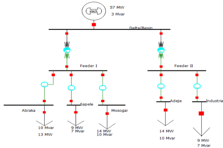
Figure 1: base network modeled in PowerWorld.
