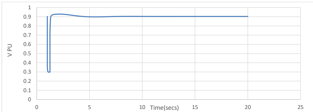
Figure 4: A plot of the per-unit Voltage against time without the connection of the Wind Turbine
