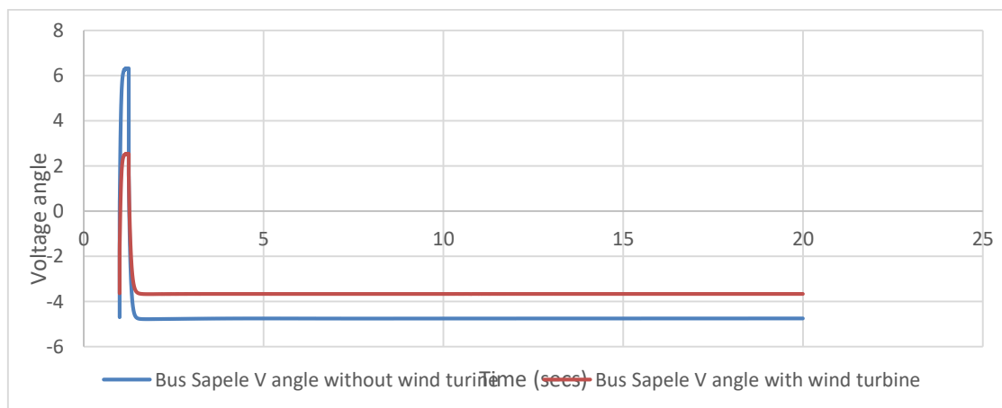
Figure 5: A plot of the voltage angle against time with the connection of the Wind Turbine
