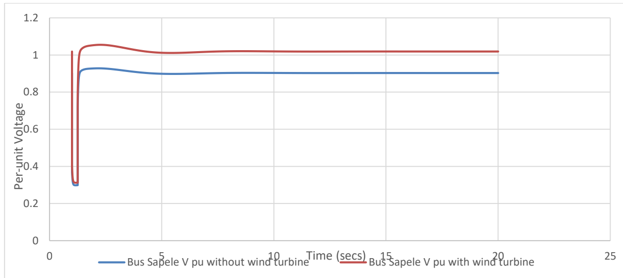
Figure 6: A plot of the voltage per-unit against time with the connection of the Wind Turbine
