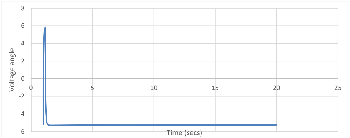
Figure 3: A plot of the voltage angle against time without the connection of the Wind Turbine
