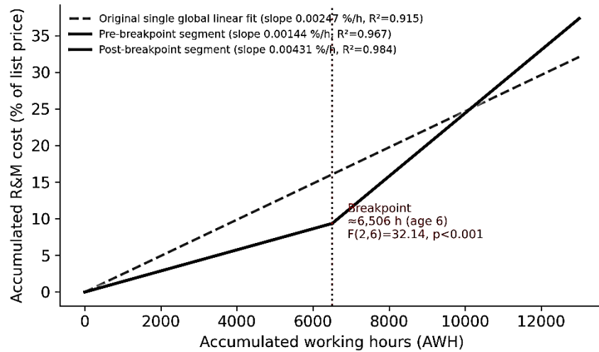
Figure 2. Gambia John Deere 5403 dataset: piecewise-fit segments vs. the original single global linear fit, reconstructed from the coefficients in Table 2 above (fitted lines shown, not raw source data points).
