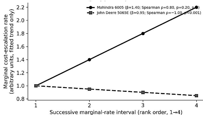
Figure 3. TOHFAN dataset: fitted marginal-rate trend by brand illustrating the accelerating (Mahindra 6005) vs. decelerating (John Deere 5065E) hazard-rate-proxy pattern implied by the \beta values in Table 3. Shown against interval rank rather than absolute hours, as the four underlying interval-hour values were not separately re-published; this is an illustrative proof-of-concept plot, consistent with Section 2.3's restriction of these results to a conceptual demonstration.
