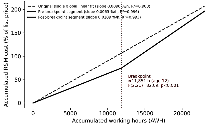
Figure 1. Kano MF375 dataset: piecewise-fit segments vs. the original single global linear fit, reconstructed from the coefficients in Table 1 above (fitted lines shown, not raw source data points, which were not re-published beyond the original study's aggregate table).
