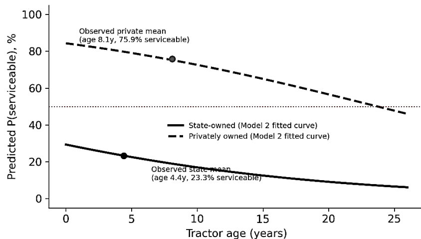
Figure 4. Delta State dataset: Model 2 fitted serviceability curves by ownership, plotted from the coefficients in Table 4 (intercept back-solved so the state-owned curve passes through the observed state mean); markers show the two groups' observed means for reference.
