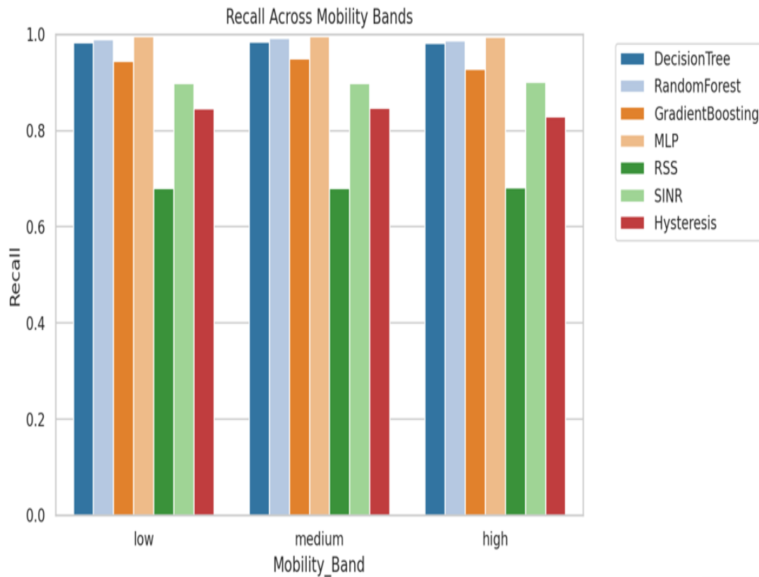
Figure 5: Plot of bar chart showing recall against mobility band
