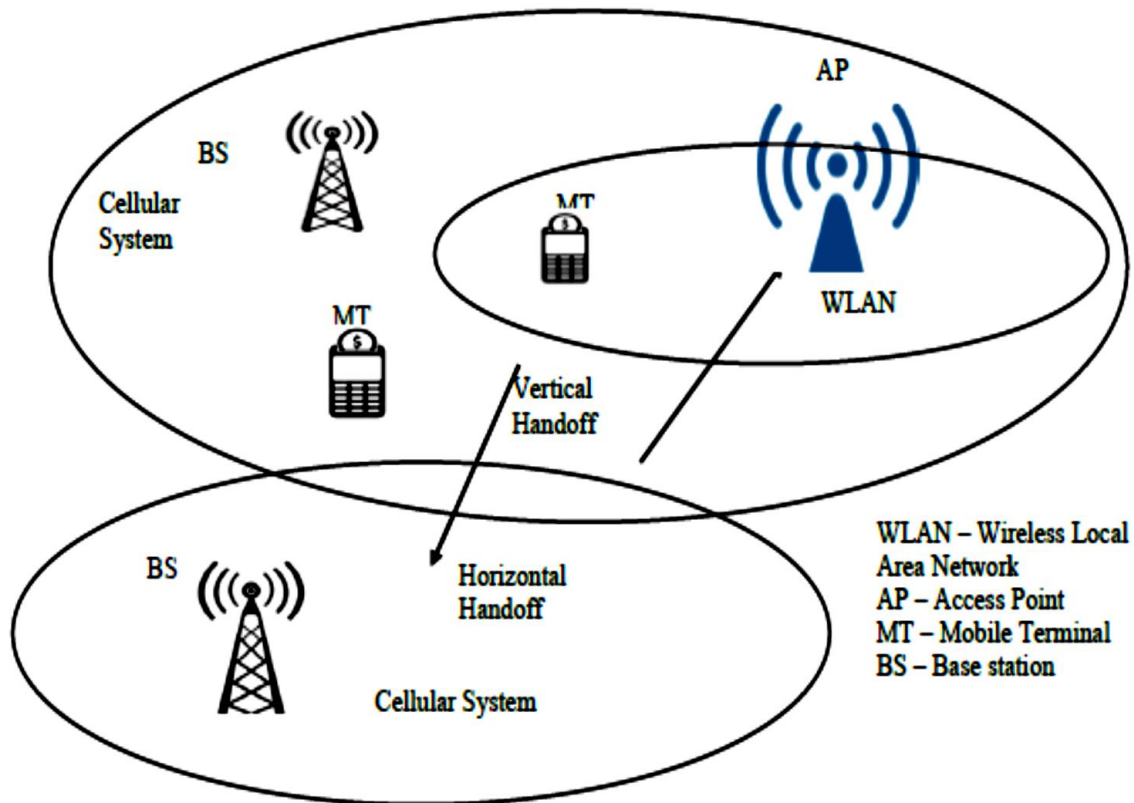
Figure 1: Diagram of a horizontal and vertical handoff
