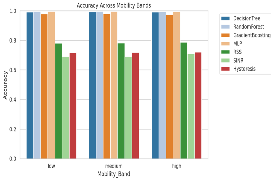
Figure 3: Plot of bar chart showing accuracy against mobility band
