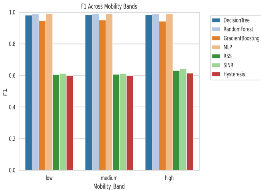
Figure 6: Plot of bar chart indicating F-1 Score against mobility band
