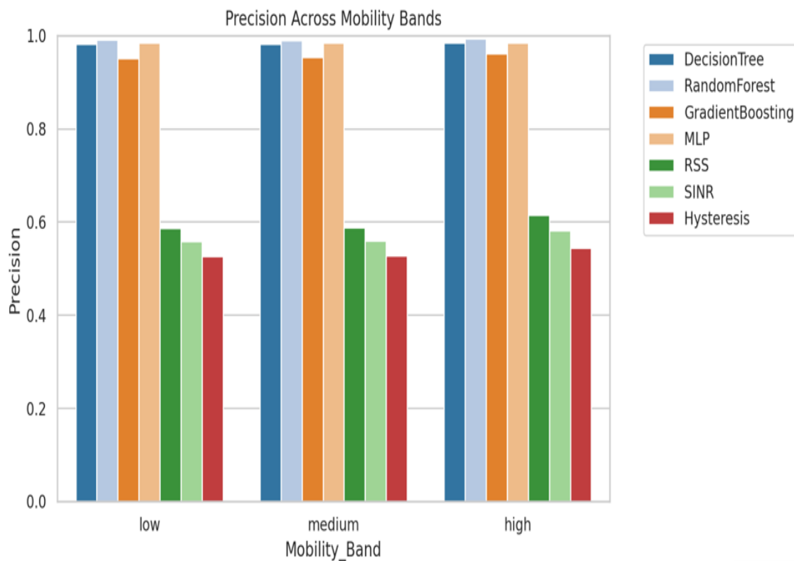
Figure 4: Plot of bar chart indicating precision against mobility band
