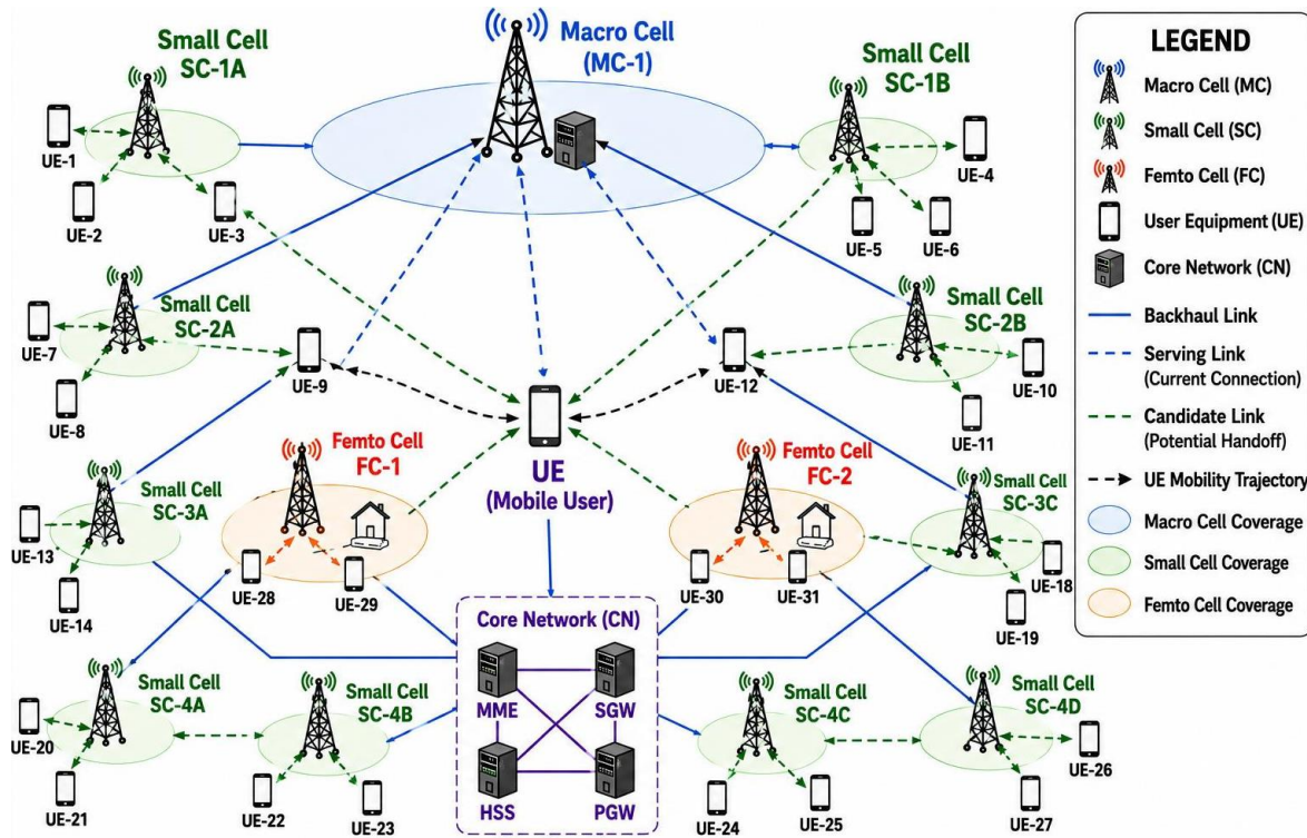
Figure 2: Design simulator for the handoff algorithm in heterogeneous network
