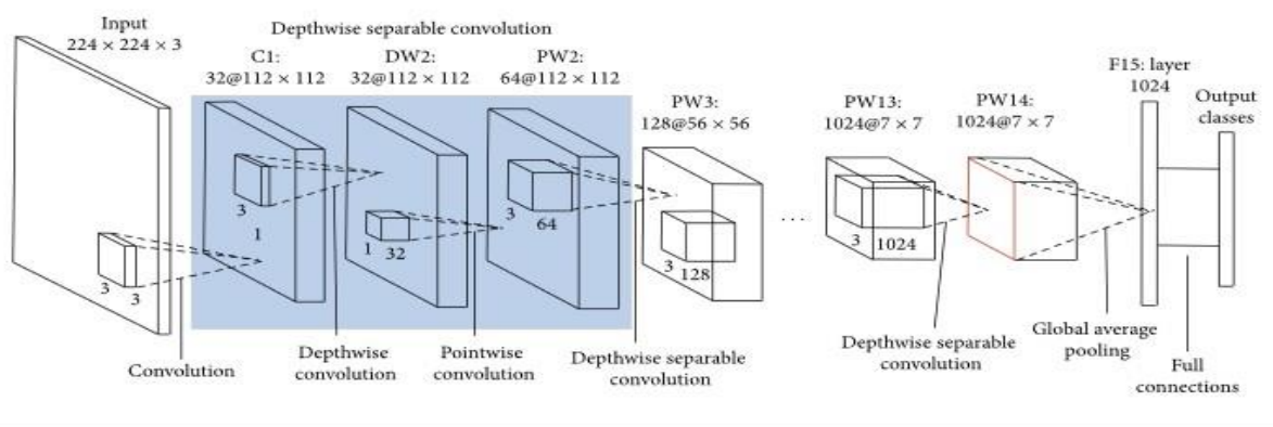
Figure 4: MobileNet-V2 + SSD architecture (Chidi et al., 2024).
