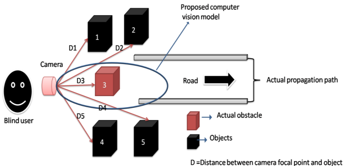
Figure 2: Proposed pipeline that couples detection with distance-based obstacle classification.
