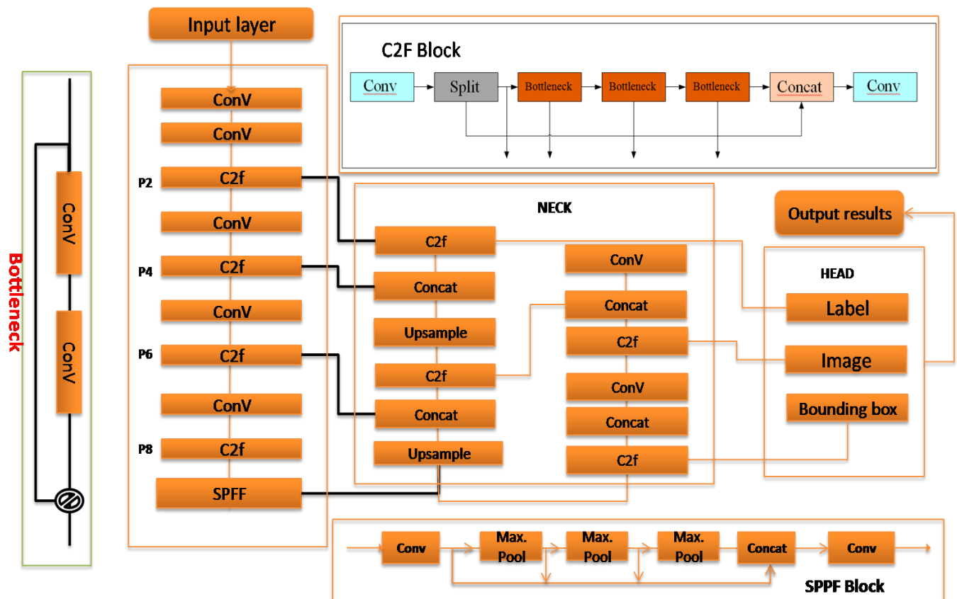
Figure 3: YOLOv8n architecture (Chidi et al., 2025).
