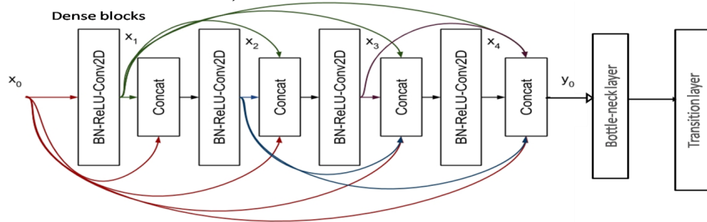
Figure 5: Block diagram of DenseNet-121.
