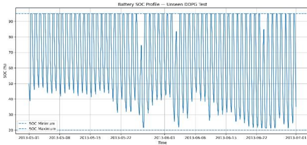
Figure 2(a): Battery State of Charge during the Unseen May–June 2013 DDPG Test Period
