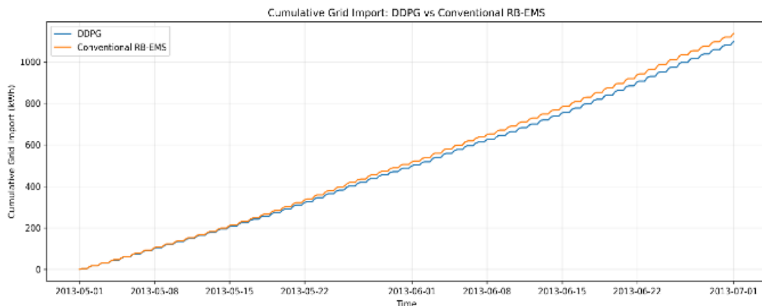
Figure 7: Cumulative Grid Import under DDPG and Conventional RB-EMS Control
