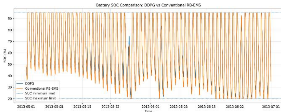
Figure 6: Comparison of Battery SOC under DDPG and Conventional RB-EMS Control
