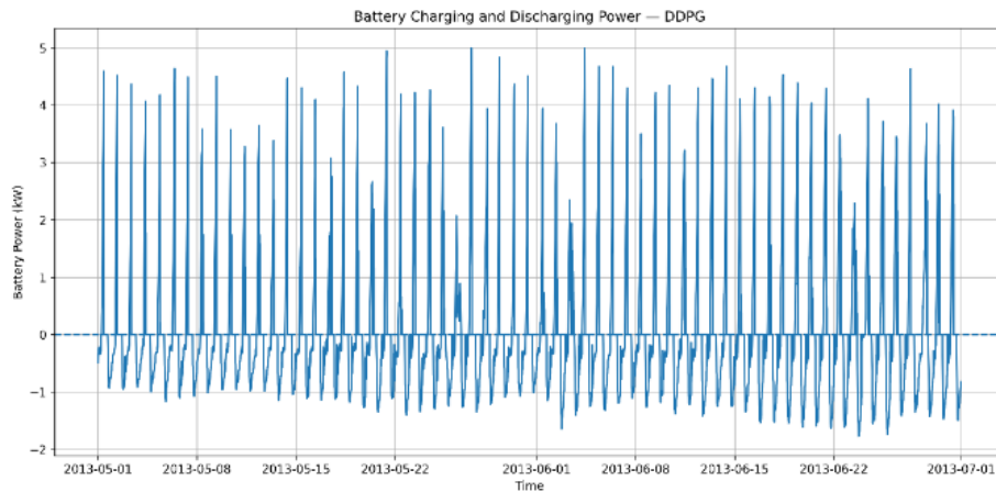
Figure 2(c): Battery Charging and Discharging Power under DDPG Control during the Unseen Test Period
