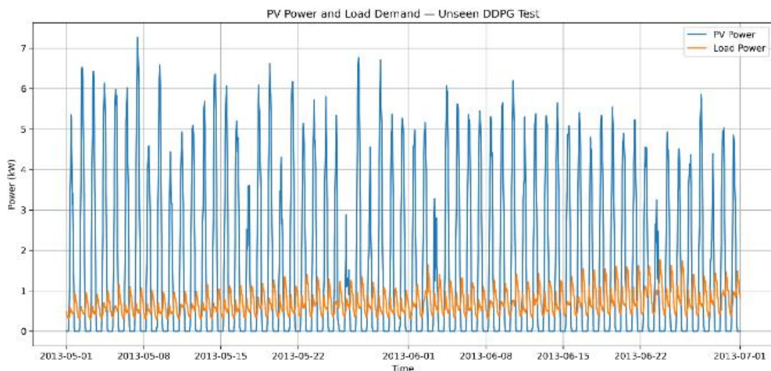
Figure 1: Photovoltaic Generation and Residential Load Demand during the Unseen May–June 2013 DDPG Test Period
