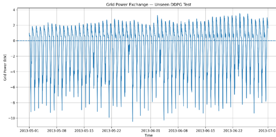
Figure 4(a): Grid Power Exchange during the Unseen May–June 2013 DDPG Test Period
