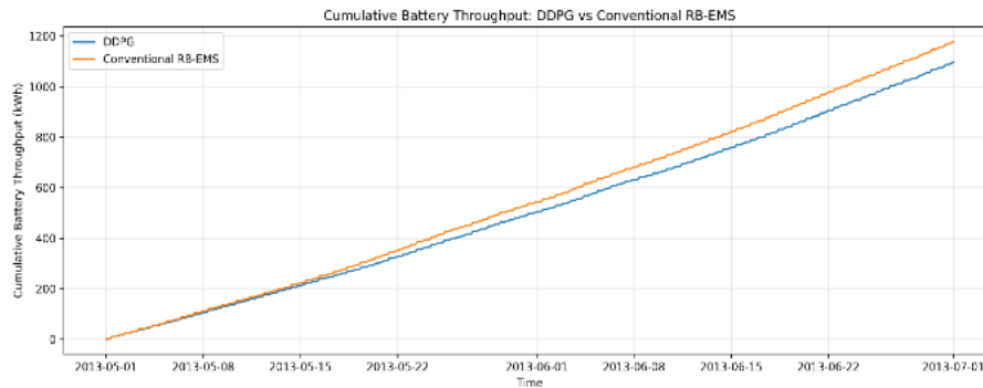
Figure 8: Cumulative Battery Energy Throughput under DDPG and Conventional RB-EMS Control
