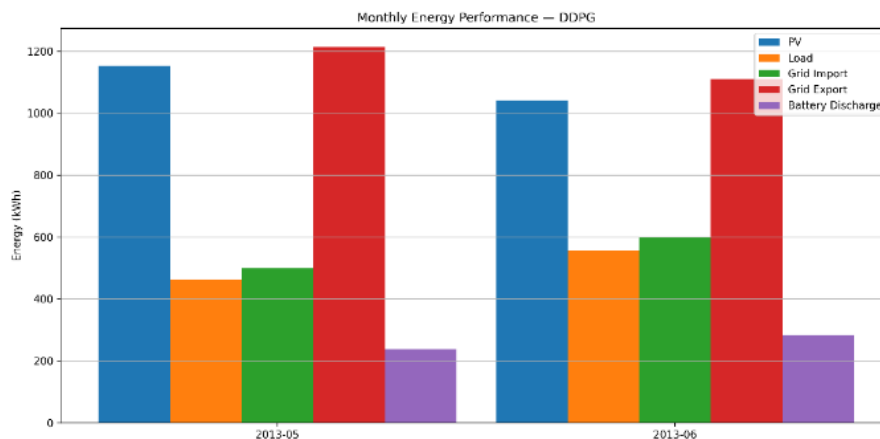
Figure 5: Monthly Energy Performance of the DDPG Controller during the Unseen Test Period
