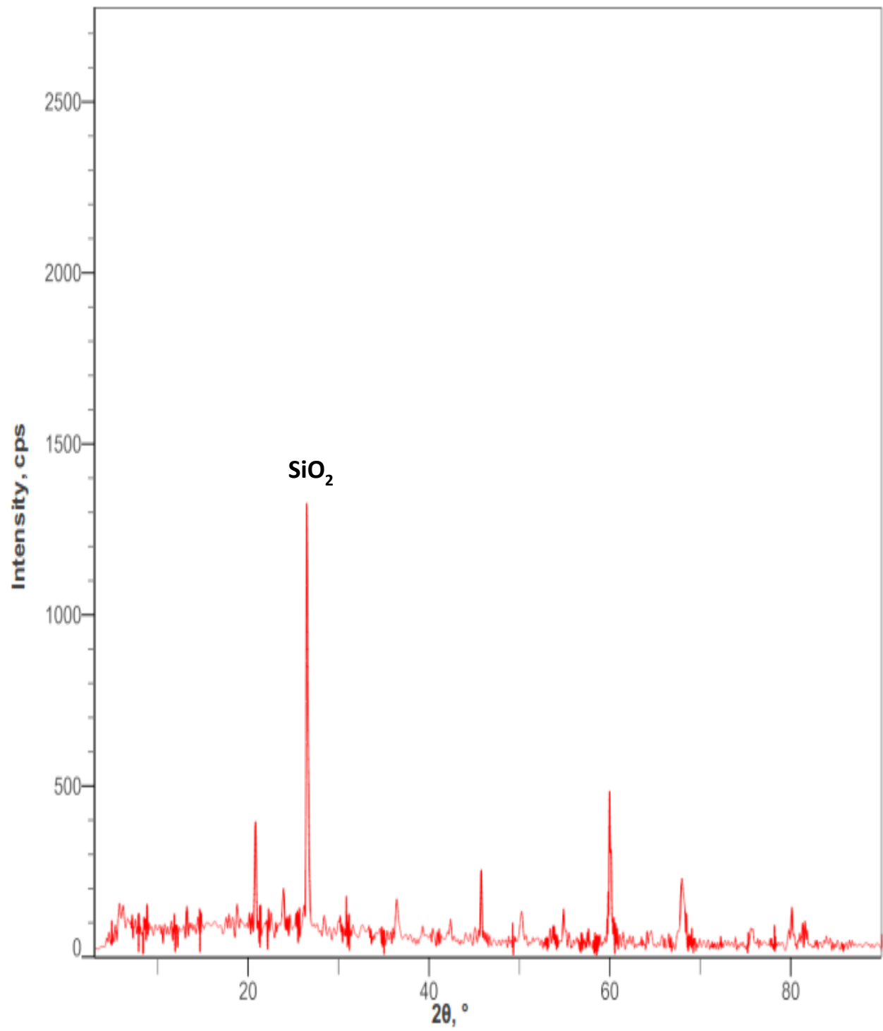
Figure 2: XRD Analysis of Nguru Soil Sample
