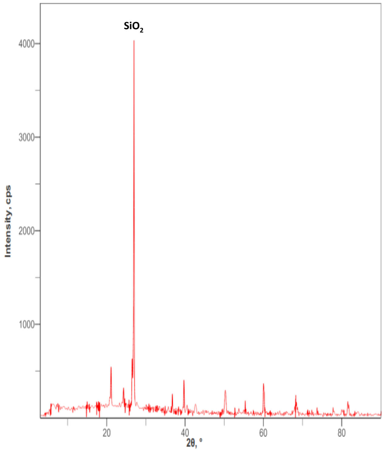
Figure 3: XRD Analysis of Karasuwa Soil Sample
