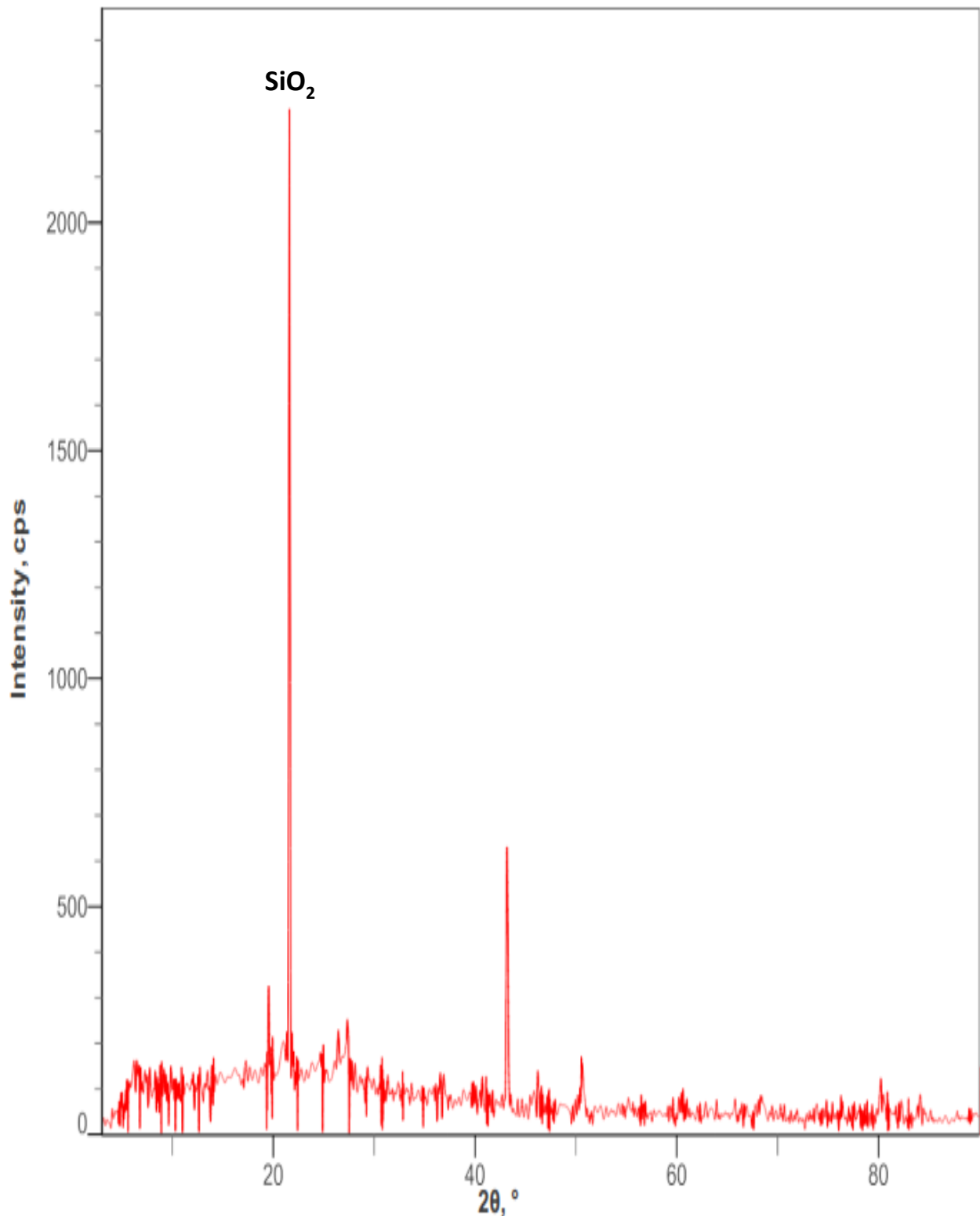
Figure 6: XRD Analysis of Machina Soil Sample
