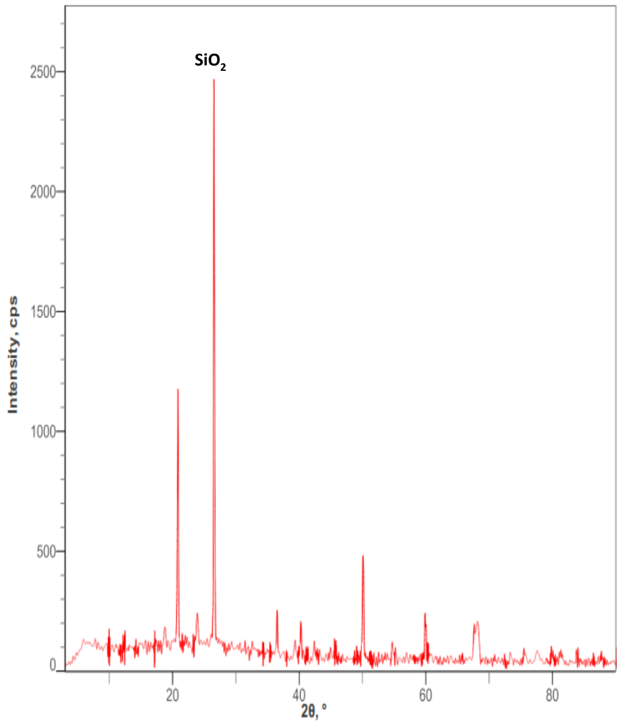
Figure 5: XRD Analysis of Jakusko Soil Sample
